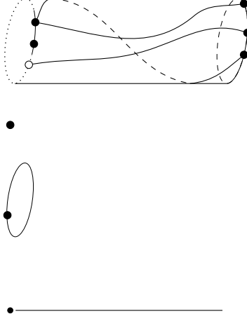
FIGURE 3. A morphism in \mathcal{Mfd}_1 , depicted as a constructible bundle over \Delta^1 .
