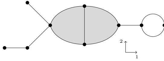
FIGURE 1. An object of \mathbf{Mfd}_2^{\text{sfr}} .
