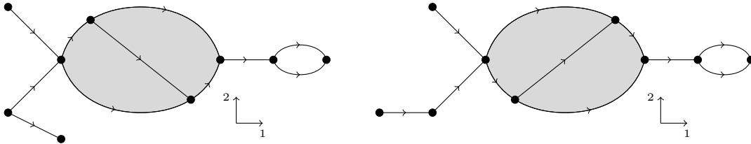
FIGURE 2. Two non-equivalent objects of \mathbf{Mfd}_2^{\mathbf{vfr}} over the same object of \mathbf{Mfd}_2^{\text{sfr}} depicted in Figure 1.
