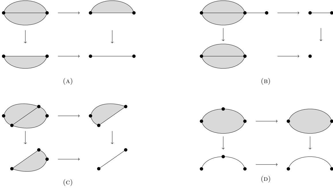
FIGURE 10. (A)–(C) depict purely closed covers; (D) depicts a refinement-closed cover. (Note: indication of the tangential structure \mathcal{B} has been suppressed in these pictures. So, strictly speaking, each of (A)–(D) depicts a diagram in \mathcal{B}\text{un} .)
