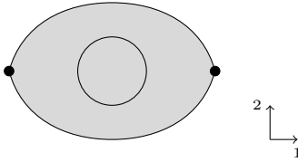
FIGURE 7. A stratified space that admits a solid 2-framing but not a vari-framing.
