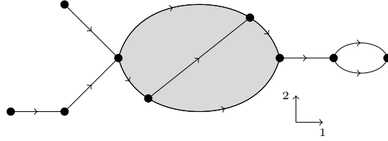
FIGURE 6. A stratified 2-vari-framed space whose underlying solid framed stratified space is the same as the underlying solid framed space of Figure 5.
