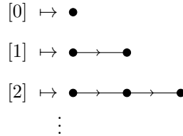
FIGURE 11. Some values of the cellular realization functor \langle - \rangle: \mathbf{\Delta}^{\text{op}} \rightarrow \mathcal{cDisk}_1^{\text{vfr}} .
