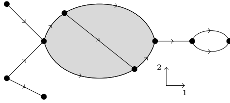
FIGURE 5. A 2-vari-framed stratified space.
