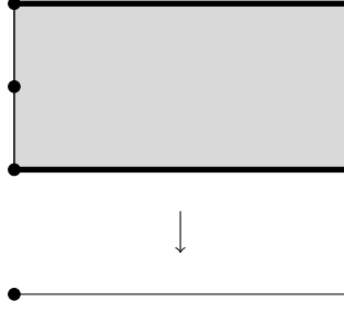
FIGURE 1. A refinement morphism in \mathbf{cBun} between two stratifications of the closed interval.
