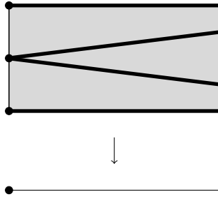
FIGURE 2. A creation morphism in \mathbf{cBun} between two stratifications of the closed interval.
