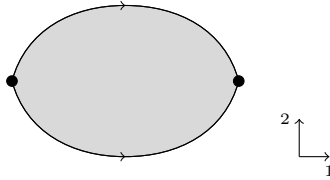
FIGURE 4. A vari-framed hemispherically stratified 2-disk.
