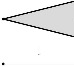
FIGURE 9. A creation morphism in \mathbf{cMfd}_1^{\text{vfr}} from \mathbb{D}^0 to \mathbb{D}^1 : see the caption for Figure 8 for how this picture indeed depicts a morphism in \mathbf{cMfd}_1^{\text{vfr}} .
