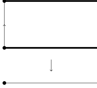
FIGURE 8. A closed morphism in \mathbf{cMfd}_1^{\text{vfr}} from \mathbb{D}^1 to \partial\mathbb{D}^0 : by definition of \mathbf{cBun} , and thereafter of \mathbf{cMfd}_1^{\text{vfr}} , a morphism is, in particular, a proper constructible bundle over the standardly stratified 1-simplex \Delta^1 = (\{0\} \subset [0, 1]) . The source, and the target, of such a morphism in \mathbf{cBun} is the fiber over \{0\} \subset [0, 1] , and over \{1\} \subset [0, 1] , respectively.
