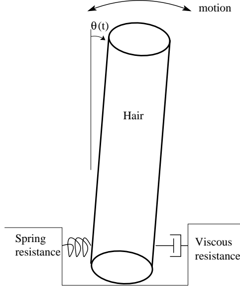
Figure 2: Inverted Pendulum Model. An early model of filiform hair motion utilized an inverted pendulum with spring- and viscous-resistance elements.
