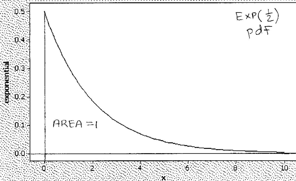
Scatterplot of exponential vs x
