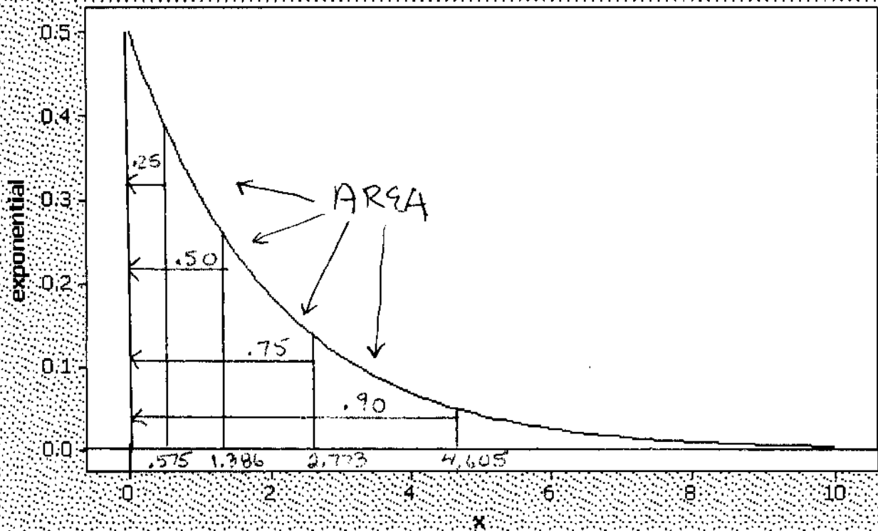
Scatterplot of exponential vs x
