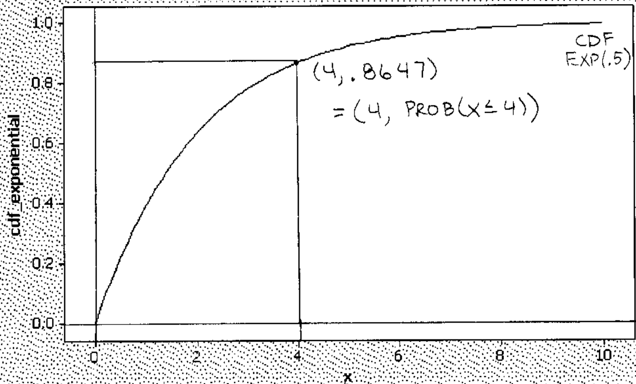
Scatterplot of cdf_exponential vs x
