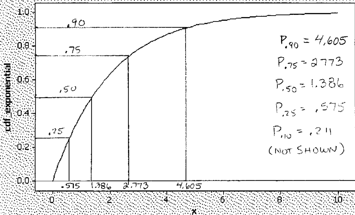
Scatterplot of cdf_exponential vs x
