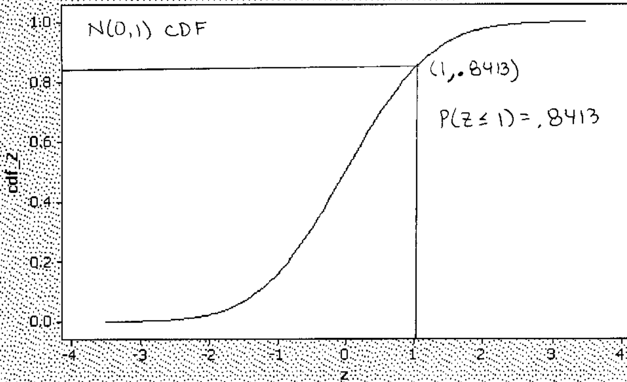
Scatterplot of cdf_Z vs z
