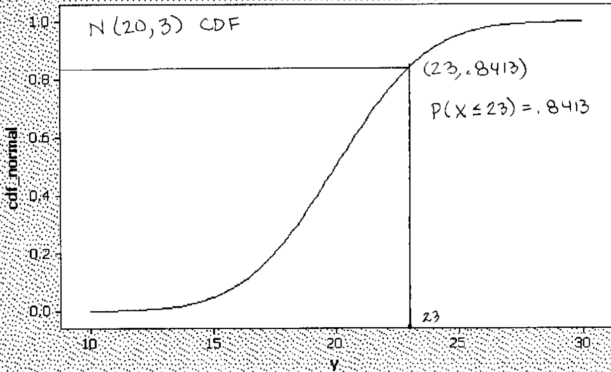
Scatterplot of cdf_normal vs y
