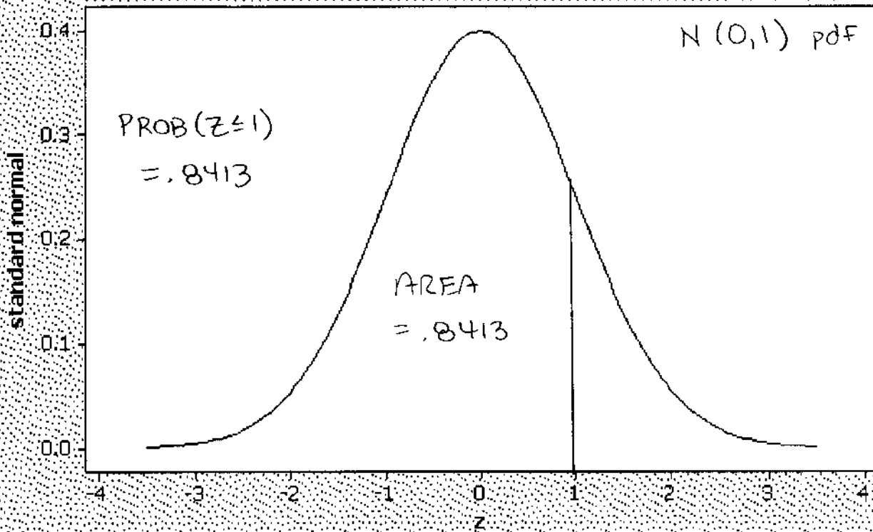
Scatterplot of standard normal vs z
