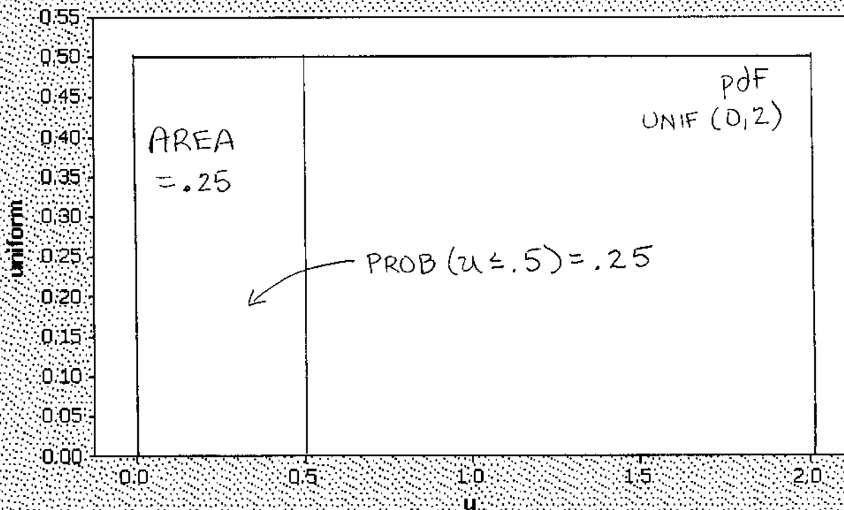
Scatterplot of uniform vs u
