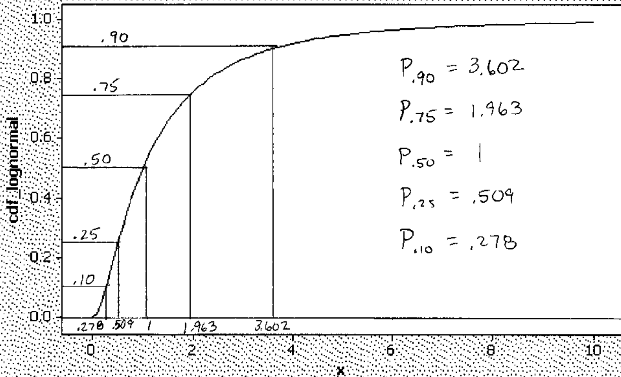
Scatterplot of cdf_lognormal vs x
