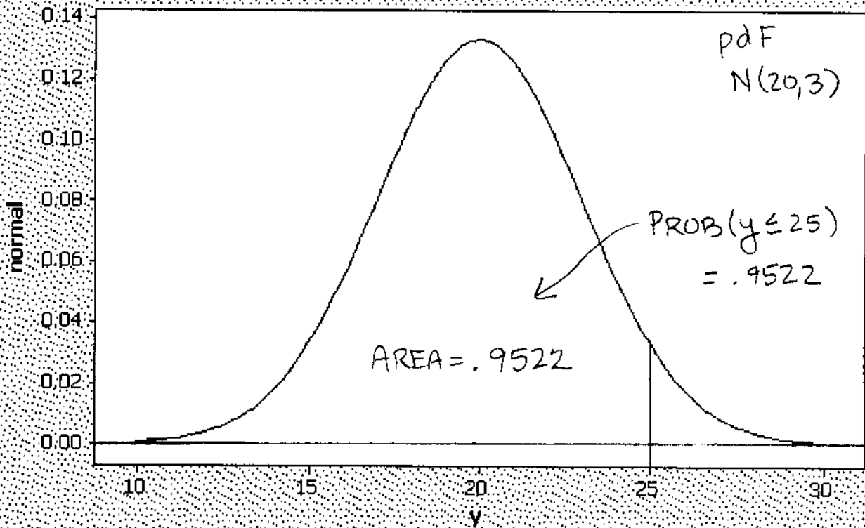
Scatterplot of normal vs y
