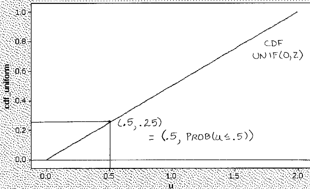
Scatterplot of cdf_uniform vs u
