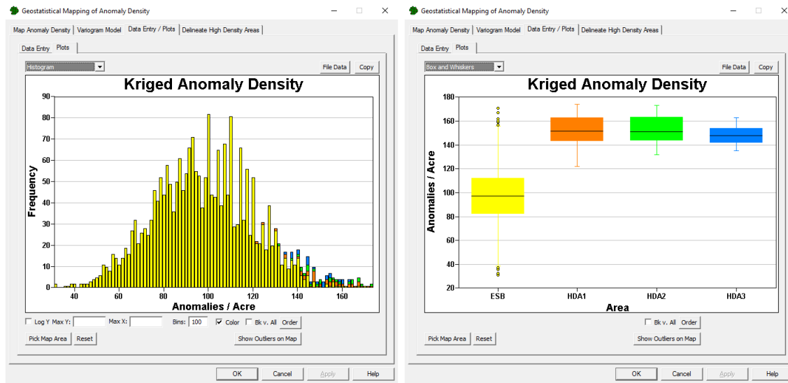
Figure 13: Visual Sample Plan plots the anomaly density in delineated regions as a histogram or boxplots. Yellow corresponds to the portion of the site not marked as a possible target area, and shows the predicted distribution of the background noise given the modeling and threshold choices made by the user.
