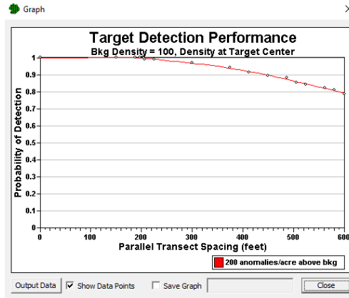
Figure 5: The VSP program window shows a detection probability curve assuming a 1,200 foot by 800 foot elliptical target area. The points on the curve were created by Monte Carlo simulation based on user-input assumptions about the size of the TA, the background anomaly density (100 anomalies per acre), and the TA anomaly density (200 anomalies per acre above the background density). The circles show the point estimates for each transect spacing that VSP simulated.
