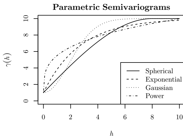
Figure 16: These semivariograms result from different parametric models for the covariance function. Each has a nugget of c_0 = 1 . The spherical, exponential, and Gaussian models have \sigma^2 = 9 and \alpha = 8 . The power model has \theta = 4.5 and \omega = 0.3 .
