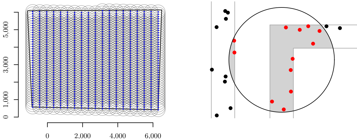
Figure 8: These diagrams illustrate the circular search windows used for calculating the local anomaly density. Left: All of these windows are used to analyze data from one sampling plan with 6 foot wide parallel transects and 390 feet of between-transect spacing. The window diameter is 800 feet. The blue points are the actual window centers generated by VSP. Right: This example shows how the window density is computed. All detected anomalies within the circle (red dots) are counted; the detected anomalies outside the circle (black dots) are ignored. The area used in the computation is the area of the intersection between the transects and the circle (shaded in grey).
