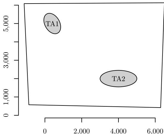
Figure 17: The easy site contains two target areas and homogeneous background anomalies. The target areas are designated TA1 and TA2. The axes on the plot are marked in feet.
