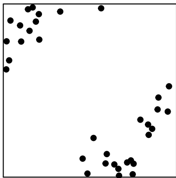
(g) A few clusters, low intensity
