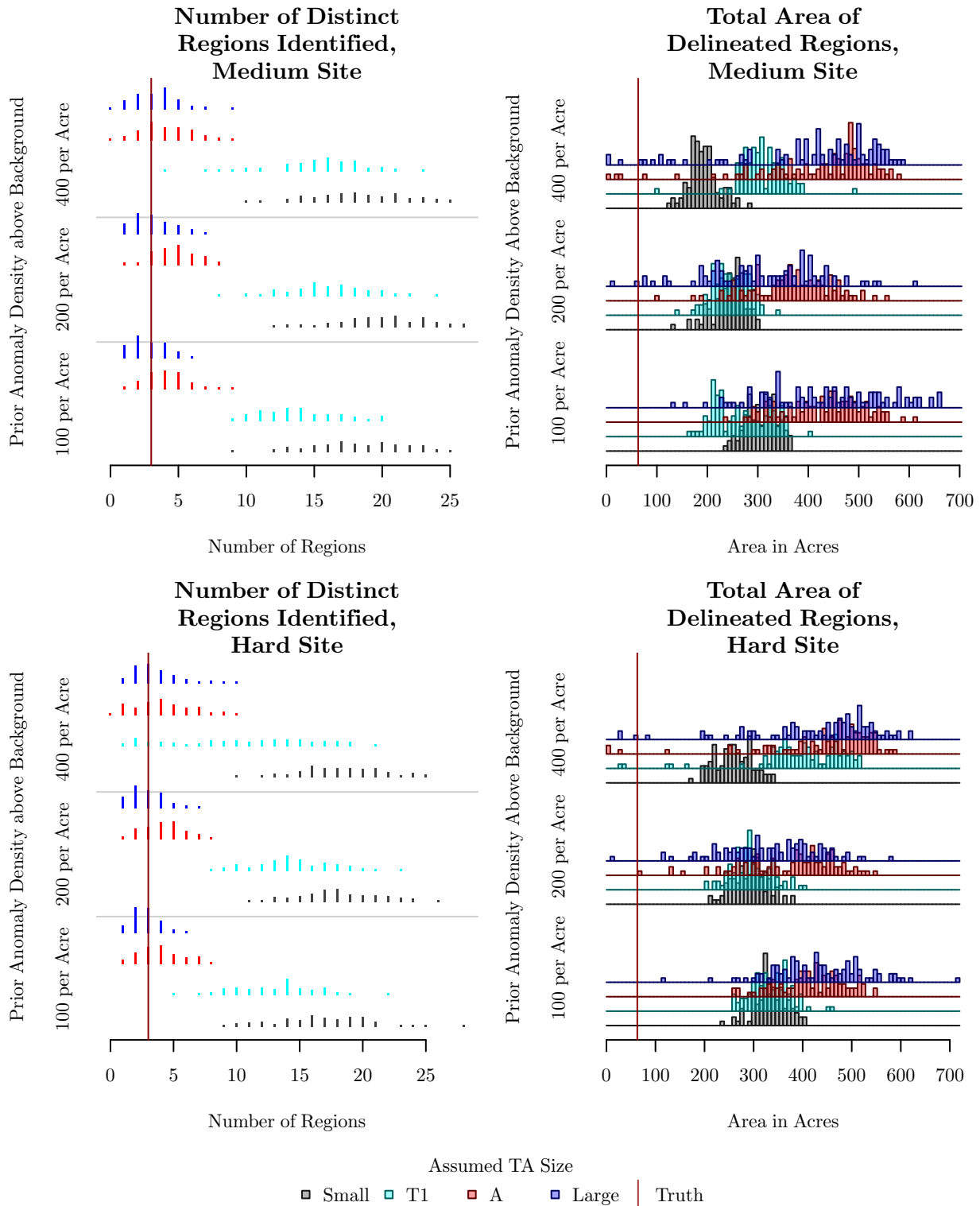
Figure 31: At the hard site, slightly more area is delineated than at the medium site, indicating that the analysis does not smooth out the clusters in the background anomalies. The vertical lines mark the true number (3) and area (62.9 acres) of the target areas.
