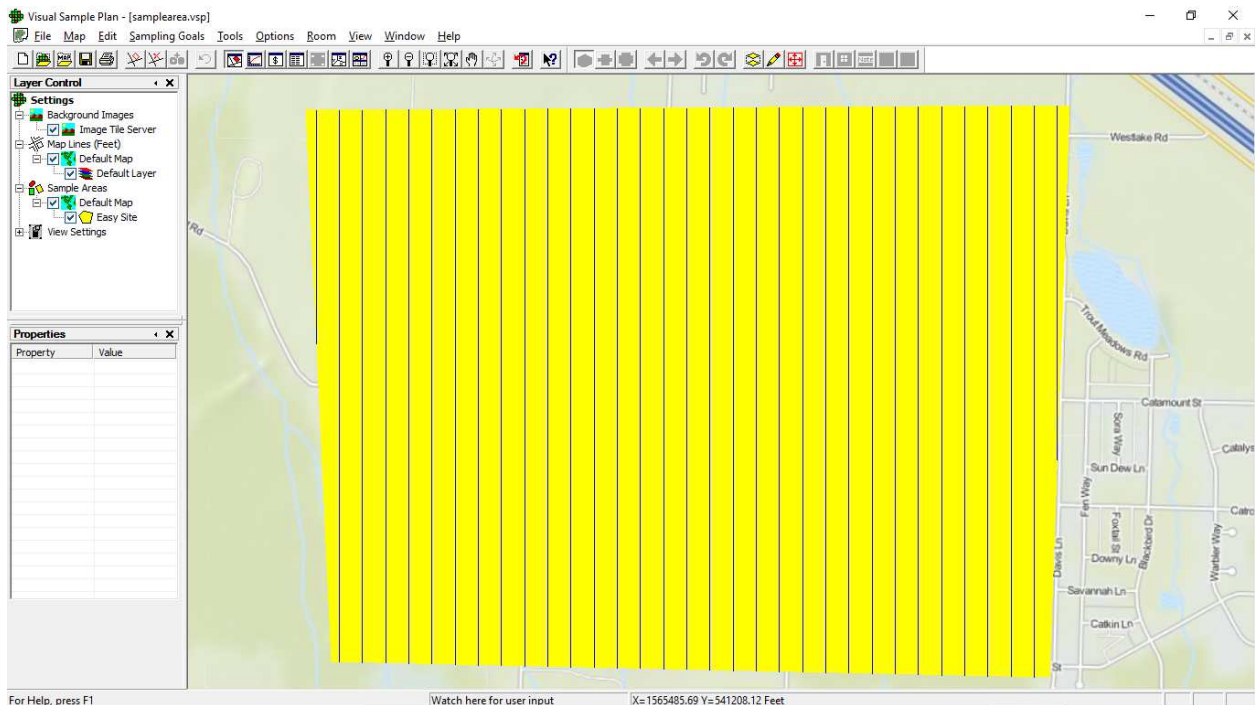
Figure 4: The VSP window shows a parallel transect sampling plan with 225 foot spacing between 6 foot wide transects.
