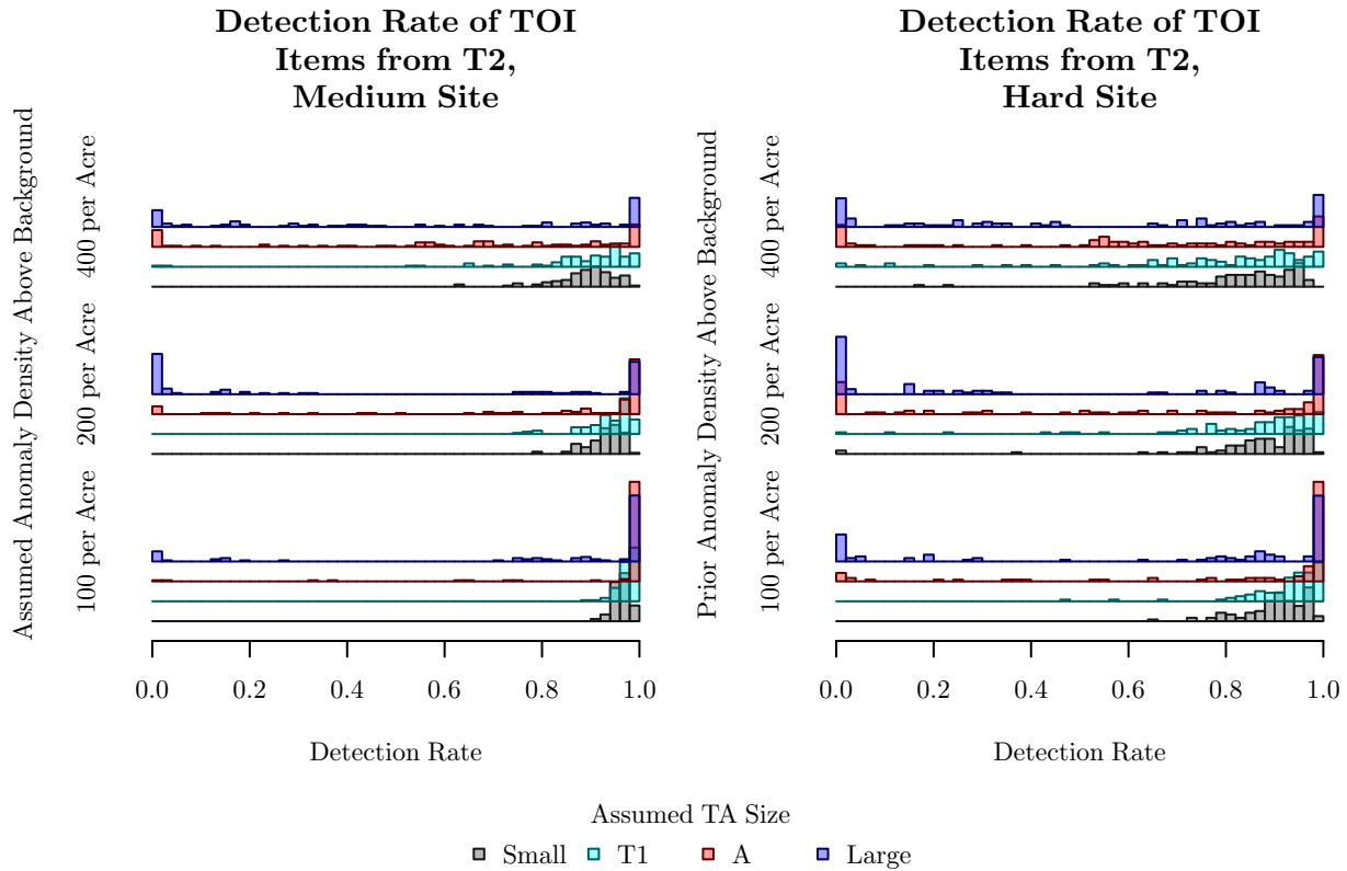
Figure 29: At both the medium and the hard site, assuming a small target area size is important for finding the third target area, T2.
