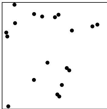
(b) Homogeneous, intensity 20
