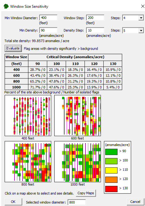
Figure 10: VSP’s window size sensitivity analysis tool summarizes the detected high-density regions graphically and in tabular form. The two smallest window diameters (400 and 600 feet) give the appearance of the site being covered in small, isolated high-density regions. In reality these are due to naturally-occurring random variation. The larger window sizes (800 and 1,000 feet) tell more reasonable stories where similar (same-colored) densities are observed in adjacent windows. The user will choose the analysis where the area of the site labeled as high-density is the most consistent with the prior information about the extent of the munitions use areas.
