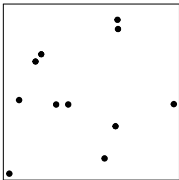
(a) Homogeneous, intensity 10
