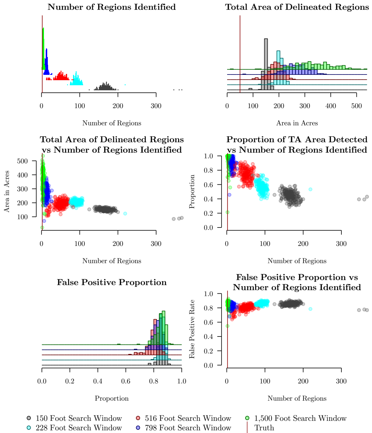
Figure 24: Plots showing the relationships between the number of regions and other variables for the window size experiment. The red vertical lines mark the true total area of the target areas (49.7 acres) and number of target areas (2).
