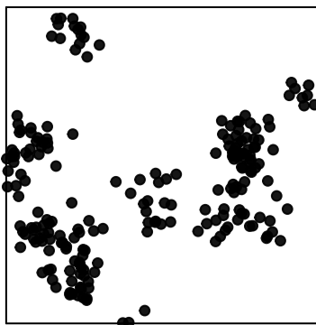
(h) More clusters, high intensity
