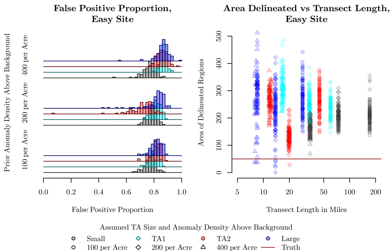
Figure 33: The easy site contains 49.7 acres of target areas, but all sampling plans result in far more area than this being delineated.
