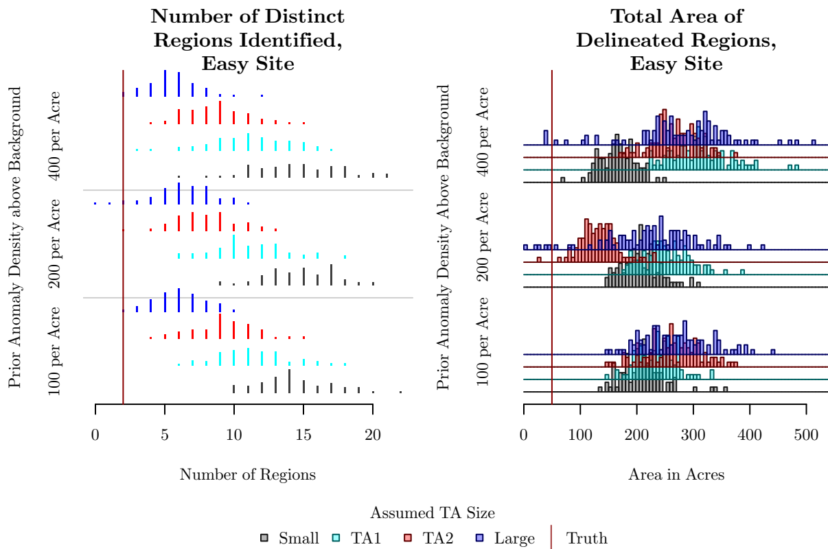
Figure 30: At the easy site, the assumed target area density has no effect on the number of regions delineated, but there is an apparent interaction between the assumed TA density and the assumed TA size. A similar pattern is seen at the medium and hard sites as well. The vertical lines mark the true number (2) and area (49.7 acres) of the target areas.
