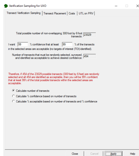
Figure 15: The user specifies a confidence level and the proportion of transects that must be free of targets of interest, and then VSP outputs a sample size.
