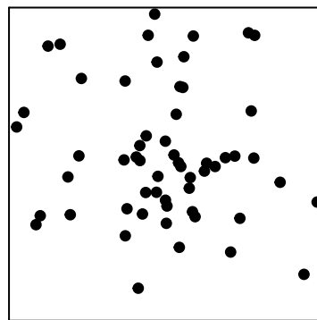
(f) Figures (c) and (e) superimposed
