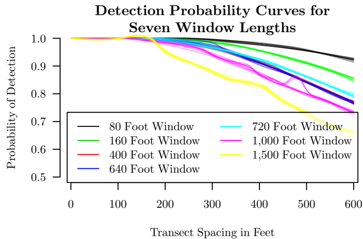
Figure 6: These detection probability curves for a 1,200 ft by 800 ft elliptical were created using Monte Carlo simulation within Visual Sample Plan. The target area is assumed to have a Gaussian distribution and 200 anomalies per acre at the center, and the background density is assumed to be 100 anomalies per acre. For each window length, ten curves illustrate the Monte Carlo error.
