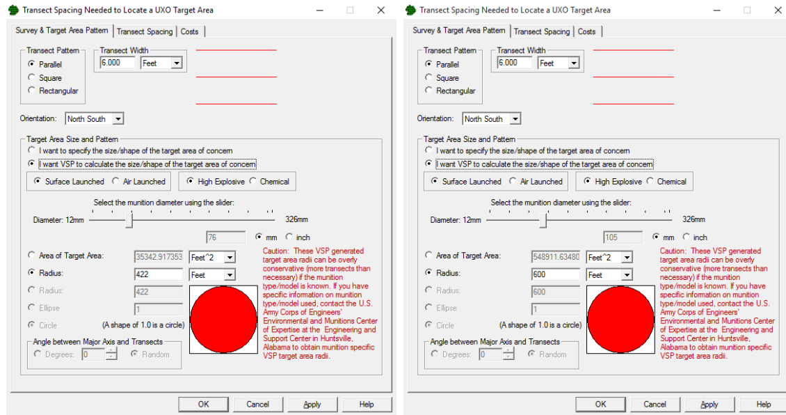
Figure 7: VSP calculates target area sizes for 76 mm and 105 mm surface-launched high-explosive shells.
