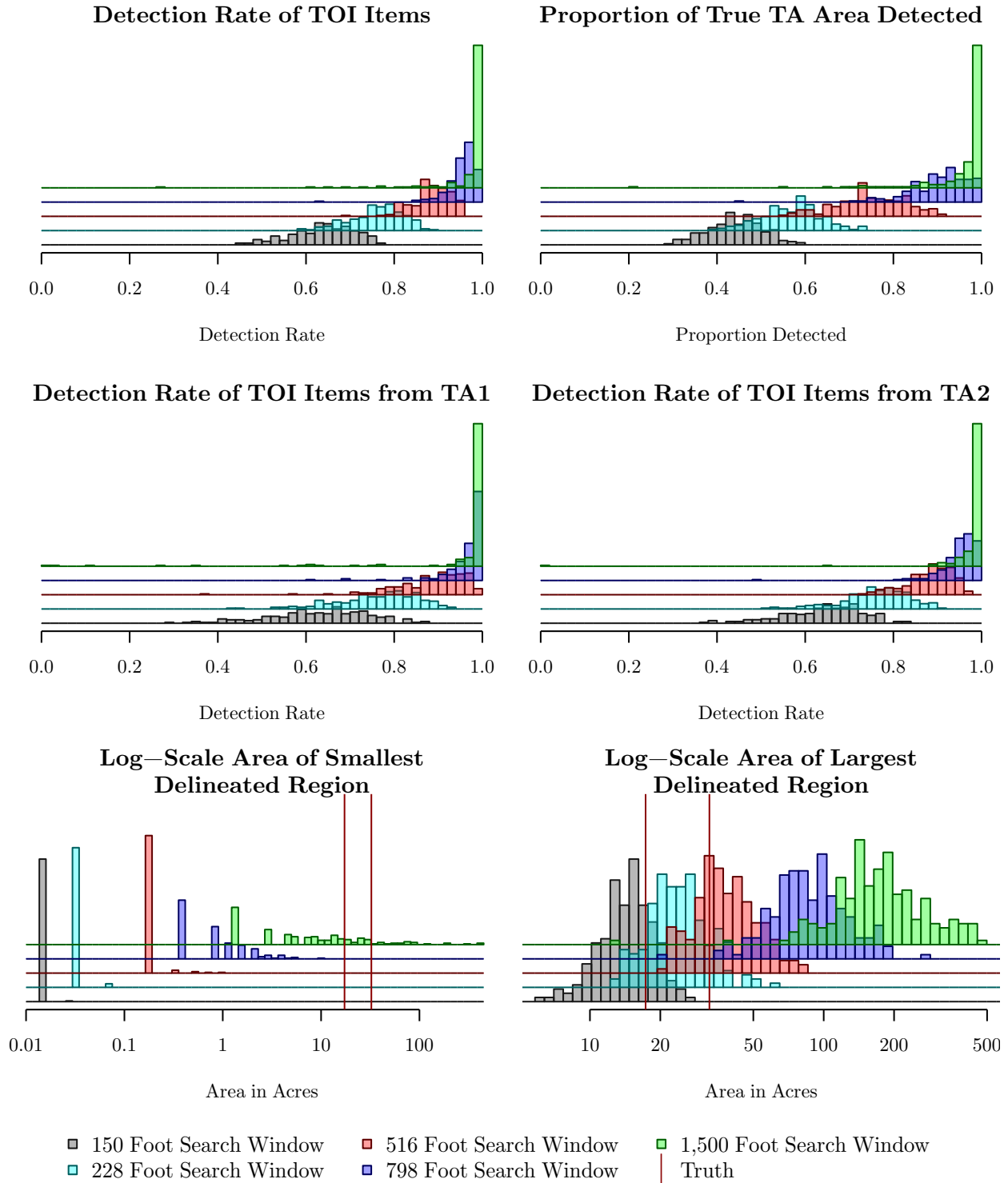
Figure 23: The detection rates and the proportion of the true area delineated measure the ability of the analysis to find the TAs and TOI items. Larger windows result in more of the TOIs being detected. The areas of the smallest and largest regions help in assessing whether the analysis produces regions that tend to be around size of the true TAs. The red lines mark the true areas of TA1 (17.3 acres) and TA2 (32.4 acres).
