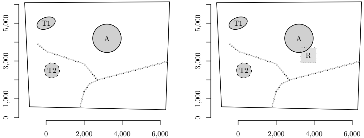
Figure 18: The medium (left) and hard (right) sites have two known target areas (T1 and A) and one unknown target area (T2), as well as a road that has elevated anomaly density. Homogeneously distributed background anomalies cover the medium site, while background anomalies at the hard site occur in clusters. The hard site contains an additional high density region due to a ranch (R) which overlaps target area A.
