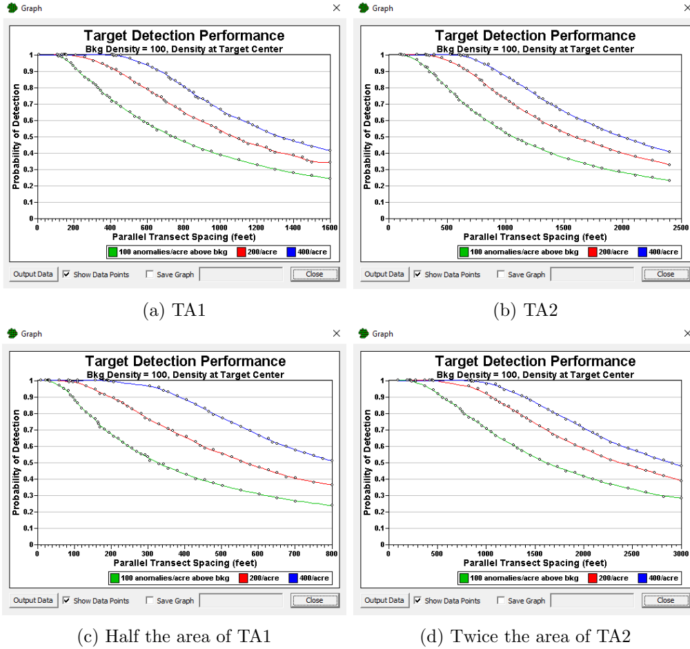
Figure 20: Visual Sample Plan created these detection probability curves by Monte Carlo simulation, based on different assumptions about the target area size and density at the easy site. These curves were used to choose the transect spacings for the sampling plans.
