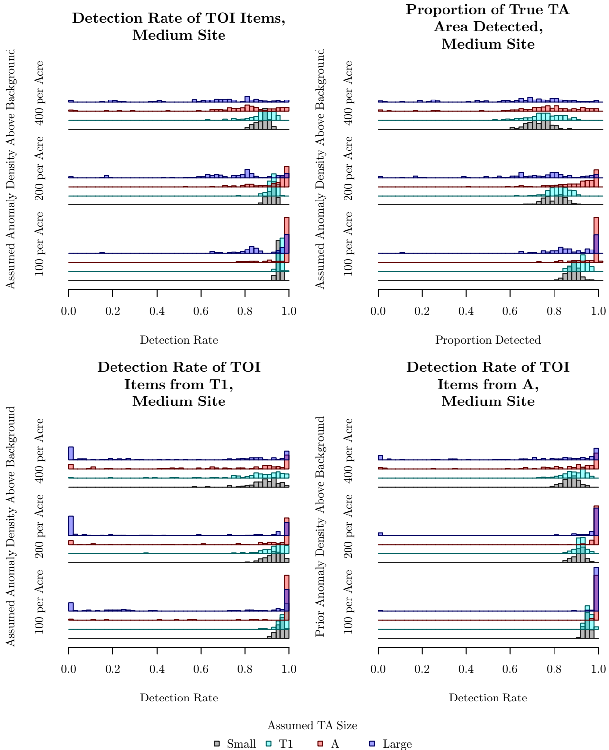
Figure 27: Compared to the easy site, detection rates at the medium site tend to be lower but show similar relationships with the assumed TA size and density.
