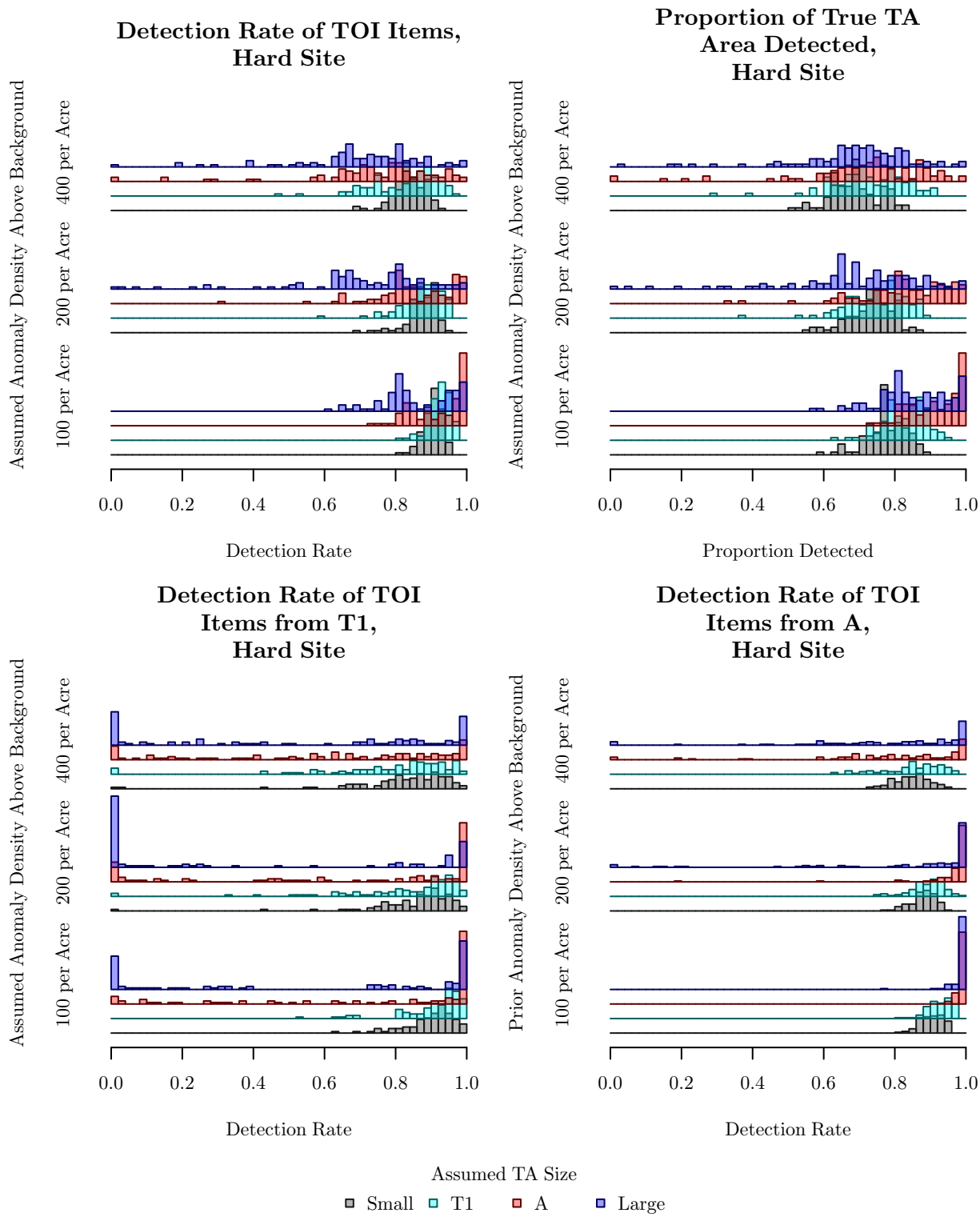
Figure 28: For the hard site, detection rates show the same trends as seen at the medium site, but the detection rates at the hard site are somewhat more variable.
