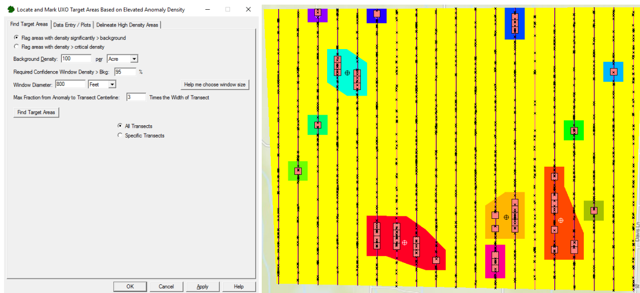
Figure 9: Left: This VSP dialog box is where the user specifies the window size and density threshold. Right: This example shows possible target areas based on 800 foot windows. The small, salmon-colored flags represent windows where the anomaly density is above 100 anomalies per acre at a 0.05 significance level. The program created the larger, colored regions are created by placing a square block at the center of each window. The transect spacing is 390 feet, so a block size of 400 ensures that blocks placed on adjacent transects can overlap. VSP creates the final result by drawing polygons around intersecting blocks.
