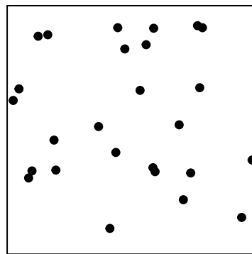
(c) Homogeneous, intensity 30
