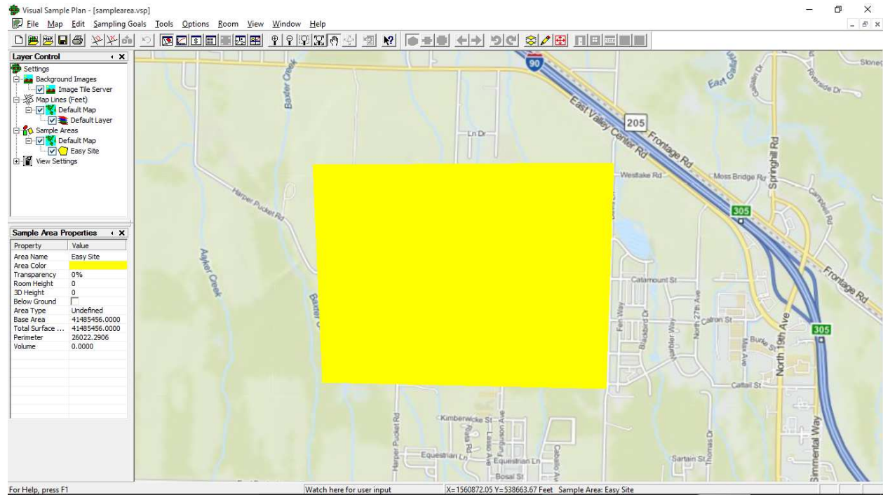
Figure 1: The VSP program window shows the site area used for the simulation study in Section 4. This is a 952.4 acre (roughly 1.4 by 1.1 mile) region situated northwest of Bozeman, Montana. A real geographic location is used only to demonstrate VSP’s map feature; the simulated sites are entirely fictitious.
