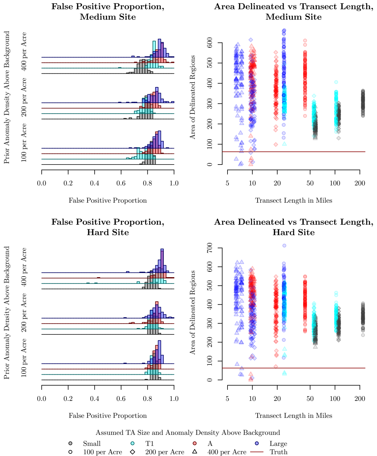
Figure 34: The medium and hard sites contain 62.9 acres of target areas. As seen at the easy site, most of the delineated area does not belong to a target area..
