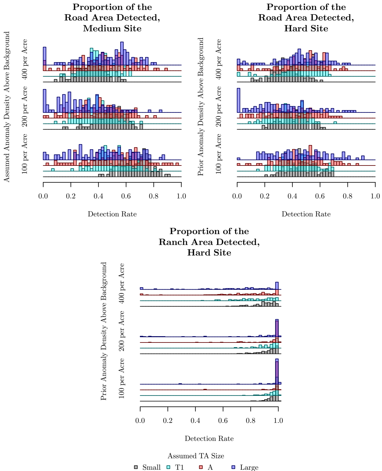
Figure 32: None of the sampling plans are able to smooth the road or the ranch out of the anomaly density map. These regions need to be described in the conceptual site model and analyzed separately.
