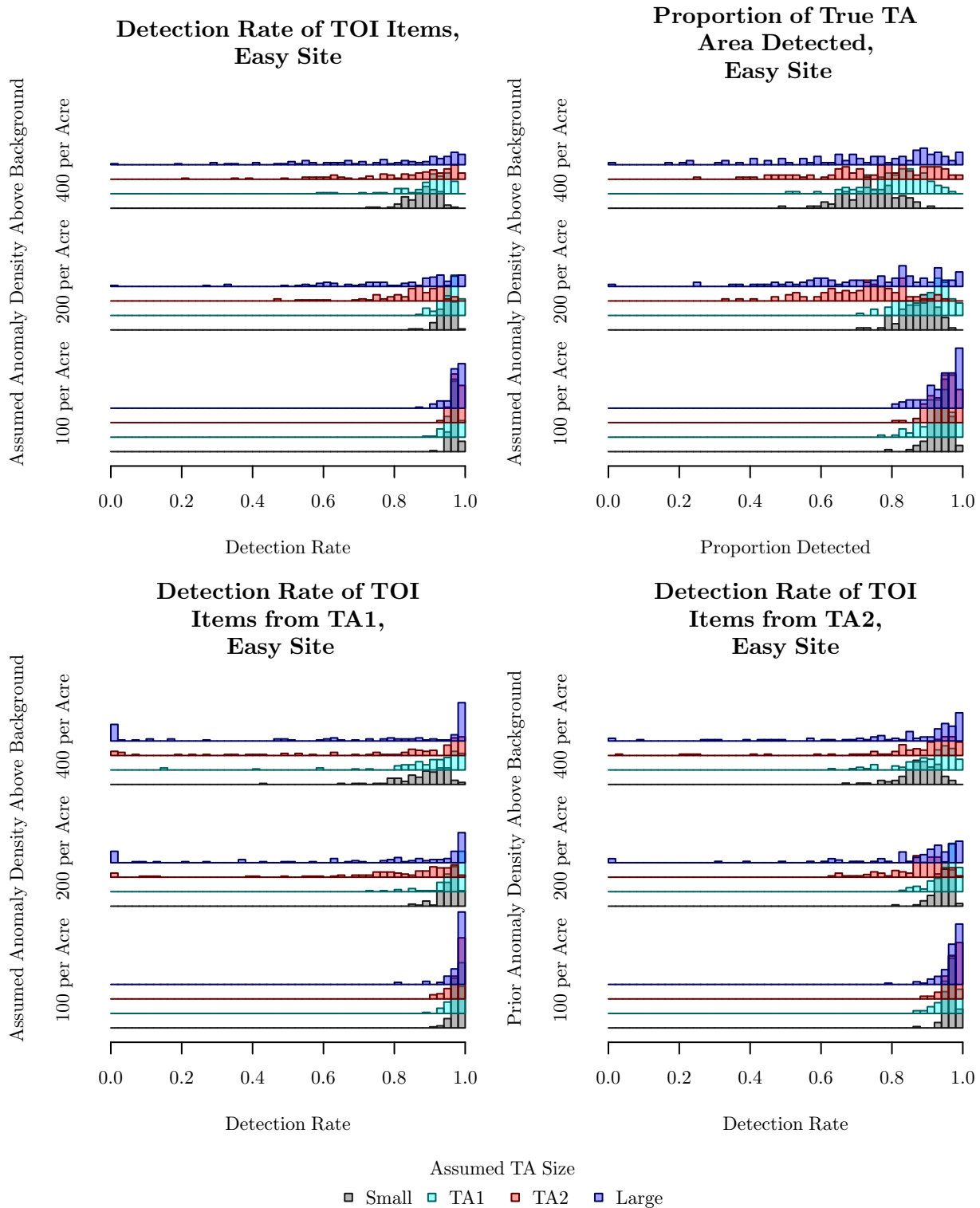
Figure 26: At the easy site, all sampling plans tend to detect most or all of the TOI items and TA area. The detection rates are more variable for larger assumed TA size and density.
