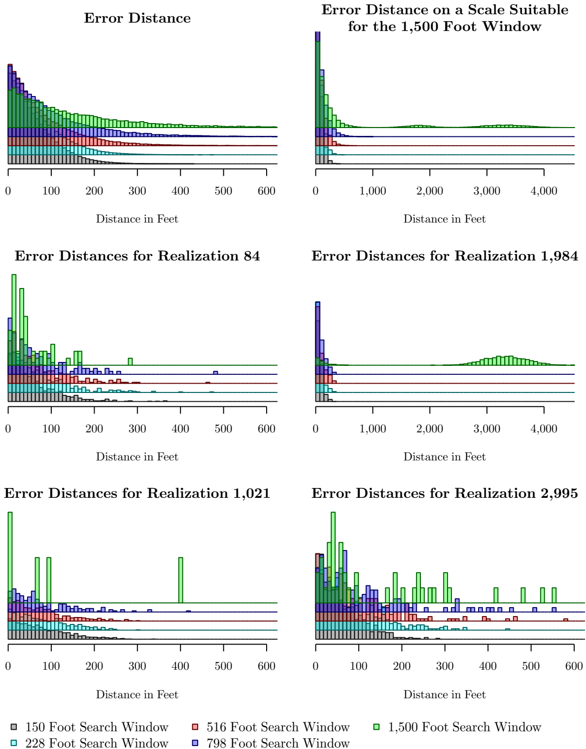
Figure 25: The distribution of error distances is right skewed both for all realizations combined and for individual realizations. Most undetected TOI items are near the boundary of a delineated region. The two clusters seen in the top right plot come from realization 1,984, where the analysis completely failed to detect TA2, and one other realization where TA1 was not detected.
