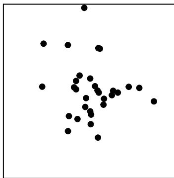
(e) Gaussian, max intensity 200
