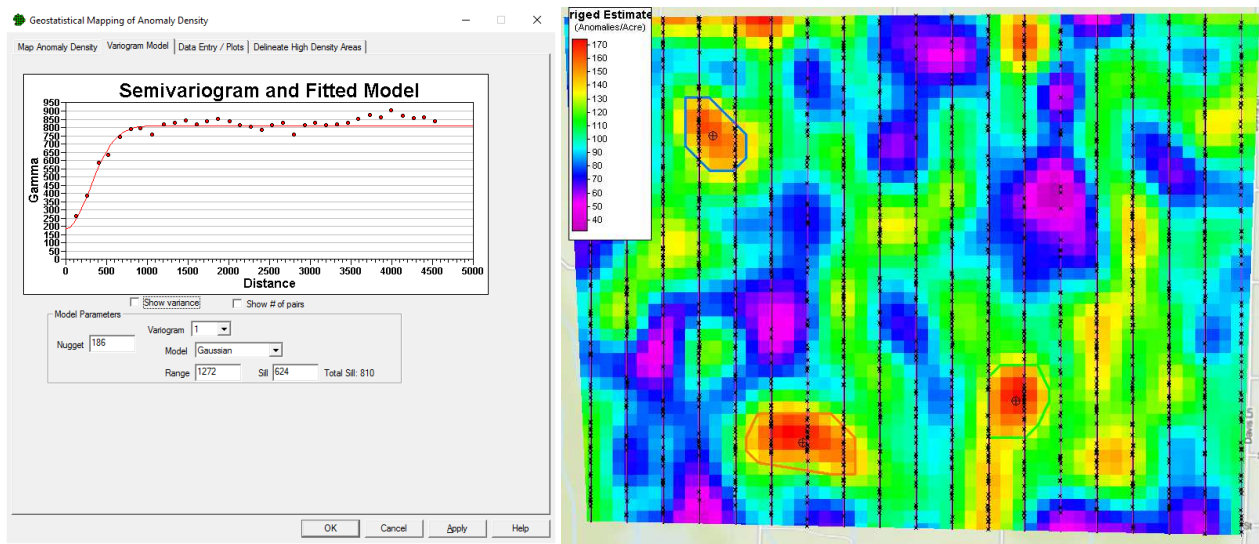
Figure 11: These example Kriging results use 800 foot windows. The transects are 6 feet wide and spaced 390 feet apart. The site contains a true 1,200 foot by 800 foot target area in the upper left and a true 2,000 foot by 900 foot target area in the lower right. Left: VSP’s semivariogram selection window shows an empirical semivariogram as points and a parametric semivariogram as a curve. Right: This anomaly density map results from Kriging with the covariance model associated with the semivariogram curve on the left. The orange, green, and blue polygons enclose sets of contiguous grid cells with estimated densities above 140 anomalies per acre and areas above 5 acres. I chose these values because they are able to separate the highest-density (red) elliptical regions from the relatively disordered-looking background (purple, blue and green). The blue polygon correctly delineates the first TA. The green polygon is at the center of the second TA, but much of the TA area is outside the polygon. The orange polygon only contains background noise.
