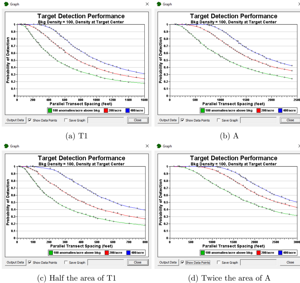
Figure 21: Visual Sample Plan created these detection probability curves by Monte Carlo simulation, based on different assumptions about the target area size and density at the medium and hard sites. These curves were used to choose the transect spacings for the sampling plans.
