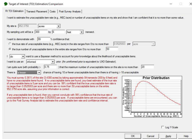
Figure 14: The user provides information to help VSP construct a prior distribution for the number of TOI items in the area. VSP then recommends a number of transects to be sampled.
